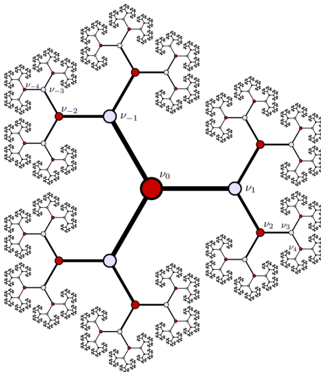
FIGURE 1. The Bruhat-Tits tree for \mathrm{SL}_2 . Source: https://ncatlab.org/nlab/files/CasselmannOnBruhatTitsTree2014.pdf (TODO: add citation).
