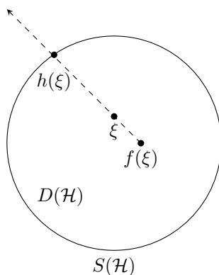
FIGURE 1. As in Hirsch's proof of the Brouwer fixed-point theorem, we construct a deformation retraction of D(\mathcal{H}) onto S(\mathcal{H}) .
