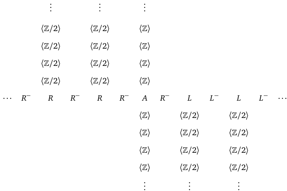
FIGURE 5. \underline{H}_{C_2}^{p,q}(S^0; A_{C_2}) , indexed by (p, p + q) .
