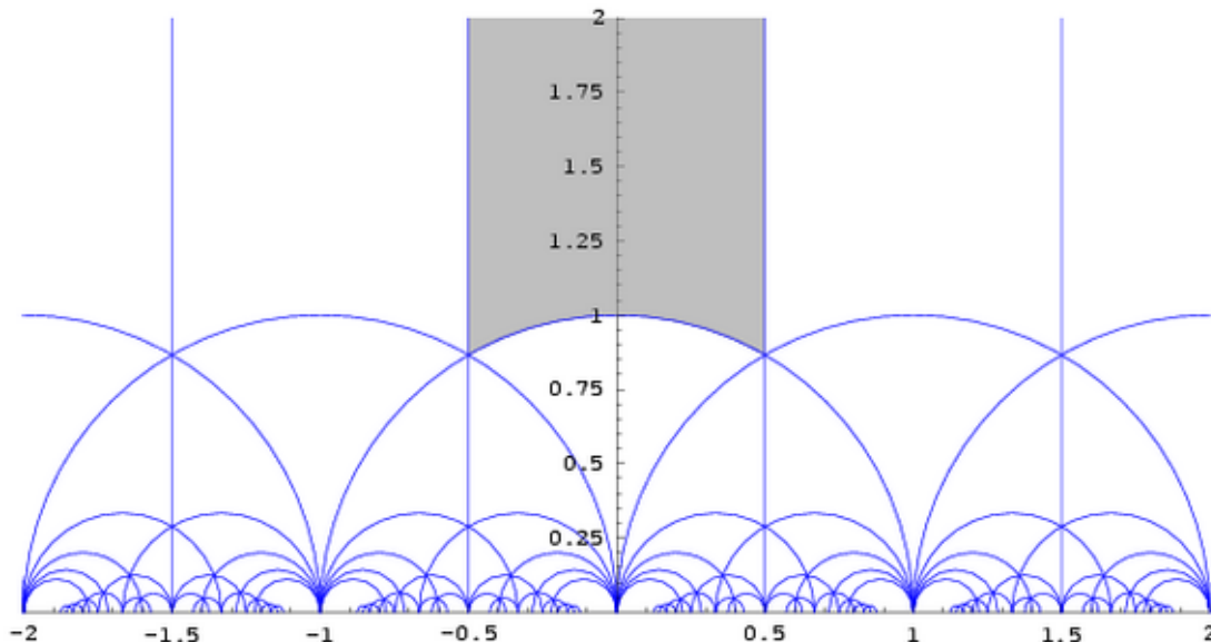
FIGURE 9. Tiling the upper-half plane with translations of \bar{\Omega} by the actions of S and T . Source: http://www.math.mcgill.ca/goren/ModularForms07-08/ModularForms.html .
