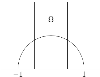
FIGURE 8. A fundamental region for \Gamma acting on \mathbb{H} , as in Theorem 21.2.
