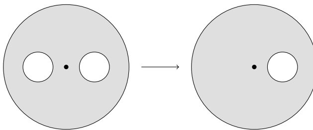
FIGURE 7. Visualizing the \mathbb{Z}/2 -action of a hyperelliptic surface.
