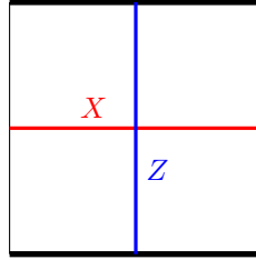
FIGURE 5. A picture of the toric code with e boundary conditions on the thick edges and m boundary conditions on the thin edges. The red line indicates an X string operator, and the blue line as a Z string operator.
